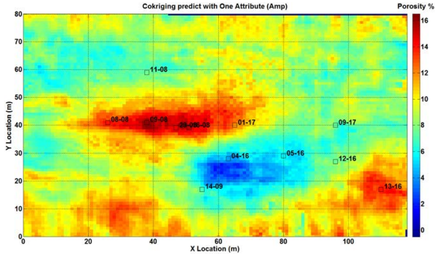
FIG. 8: Traditional cokriging prediction with seismic amplitude
