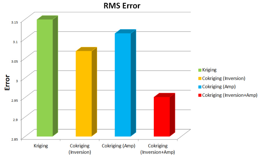
FIG. 10: Leave-one-out Cross-validation
