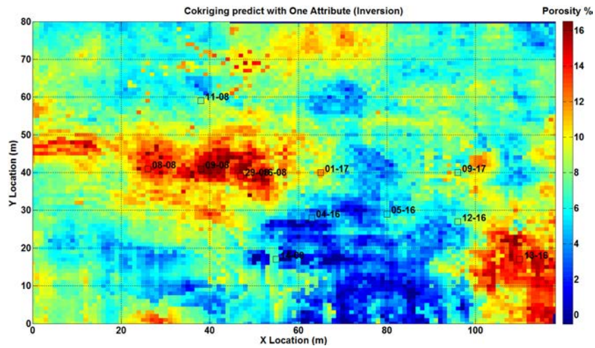
FIG. 7: Traditional cokriging prediction with inversion
