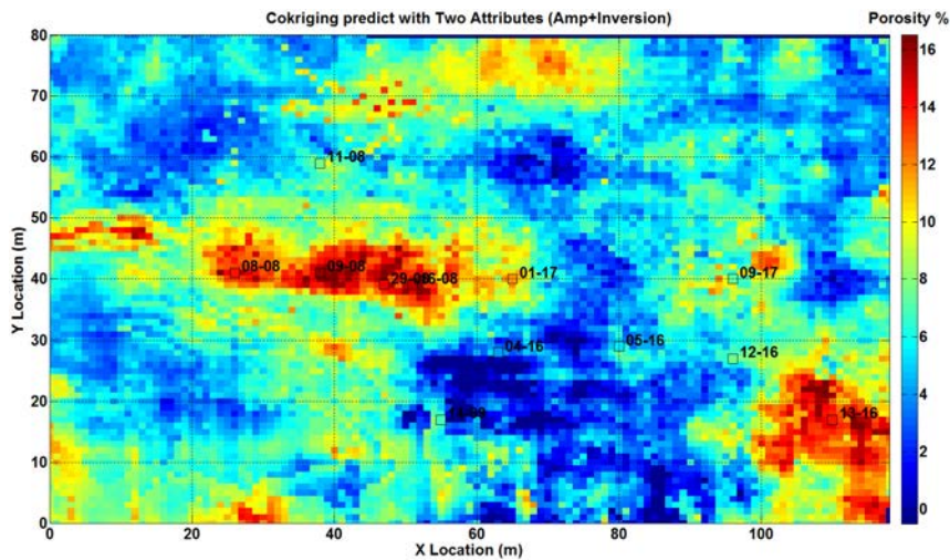
FIG. 9: Cokriging prediction with two secondary data (inversion and seismic amplitude)
