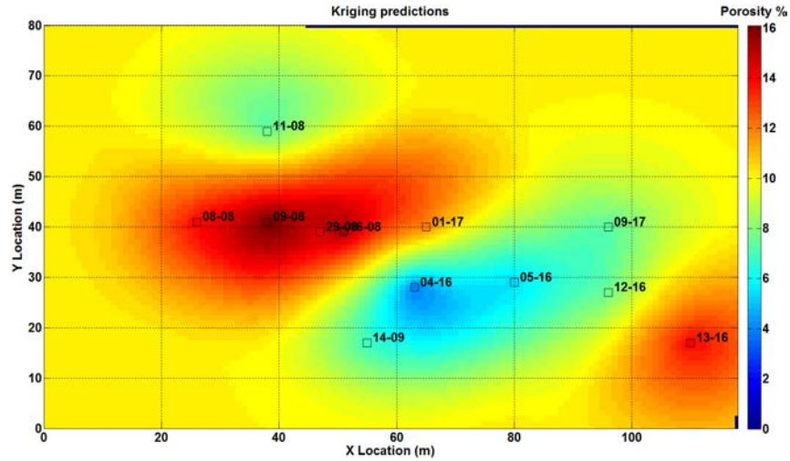
FIG. 6: Kriging interpolation with well log data
