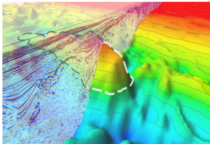
The same high / horst and a seismic line crossing it are shown in a 3D view.
